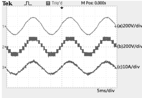
Fig. 9 experimental results for the AC side of the seven-level inverter, (a) utility voltage, (b) output voltage of seven-level inverter, (c) output current of seven-level inverter.
