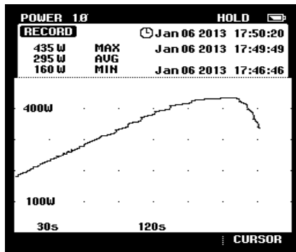
Fig. 12 output power scan of the solar cell array.
