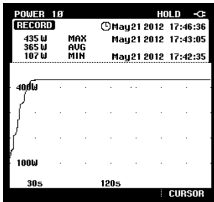
Fig. 13 experimental results for the MPPT performance of the proposed solar power generation system.
