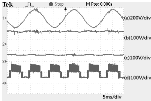
Fig. 10 experimental results for the DC side of the seven-level inverter, (a) utility voltage, (b) voltage of capacitor C_2 , (c) voltage of capacitor C_1 , (d) output voltage of capacitor selection circuit.
