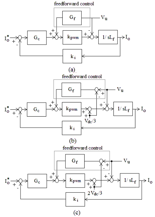
Fig. 5 model of seven-level inverter under different range of utility voltage, (a) in the range of smaller than V_{dc}/3 , (b) in the range of (V_{dc}/3, 2V_{dc}/3) , (c) in the range of higher than 2V_{dc}/3 .
