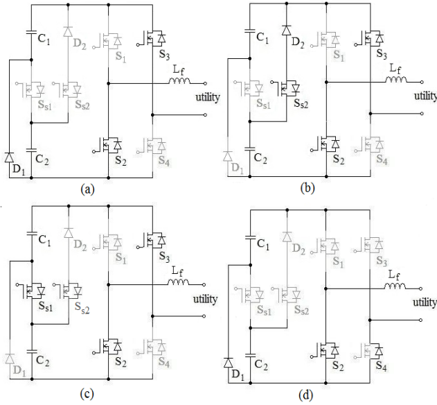
Fig. 4 operation of seven-level inverter in the negative half cycle, (a) mode 5, (b) mode 6, (c) mode 7, (d) mode 8.
