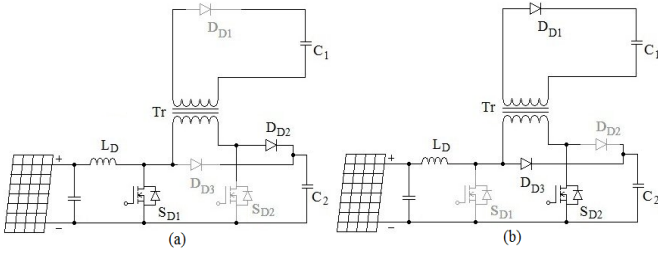
Fig. 2 operation of DC-DC power converter, (a) S_{D1} is on, (b) S_{D1} is off.
