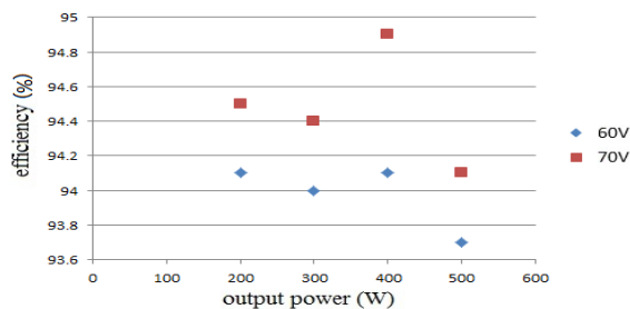
Fig. 14 experimental results for the power efficiency of the proposed solar power generation system.
