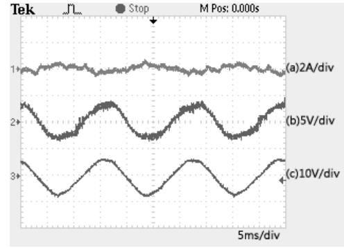
Fig. 11 experimental results of the DC-DC power converter, (a) ripple current of inductor, (b) ripple voltage of capacitor C_2 , (c) ripple voltage of capacitor C_1 .
