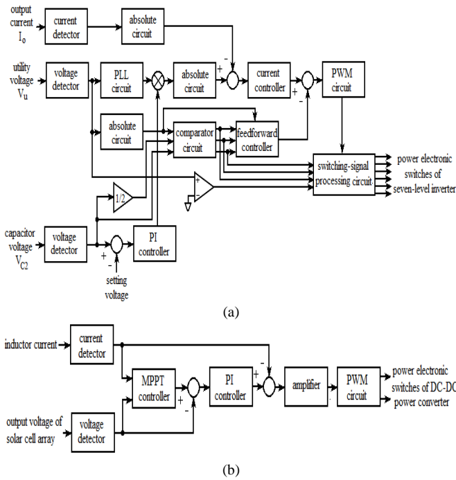
Fig. 8 control block, (a) seven-level inverter, (b) DC-DC power converter.
