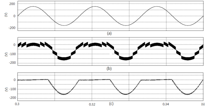
Fig. 7 simulation results of proposed solar power generation system, (a) utility voltage, (b) negative terminal voltage for adding the symmetric filter inductor, (c) negative terminal voltage for adding the symmetric filter inductor and the extra filter C_f-R_f-C_f .
