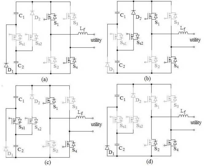
Fig. 3 operation of seven-level inverter in the positive half cycle, (a) mode 1, (b) mode 2, (c) mode 3, (d) mode 4.
