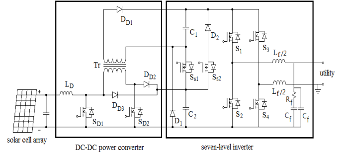
Fig. 6 configuration of the proposed solar power generation system for suppressing the leakage current.
